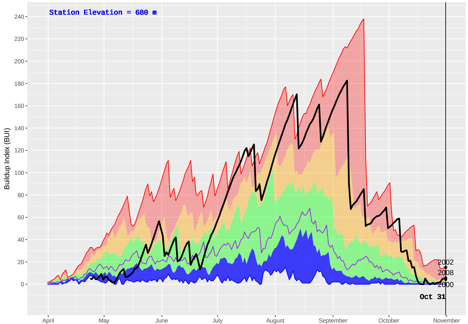
REVELSTOKE (363) : Historical (1995–2016) and Current (2017) Noon Buildup Index (BUI)
