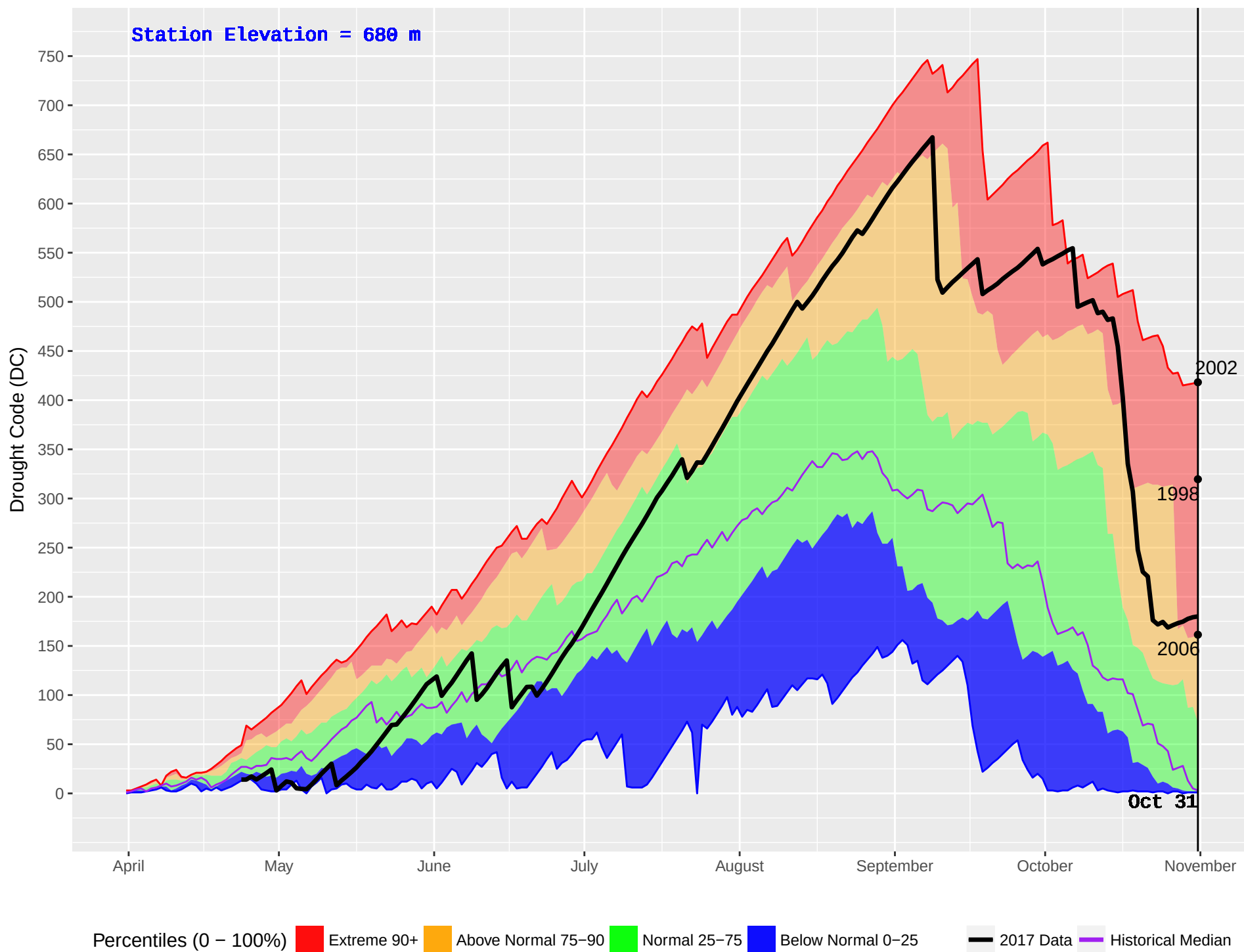
REVELSTOKE (363) : Historical (1995–2016) and Current (2017) Noon Drought Code (DC)
